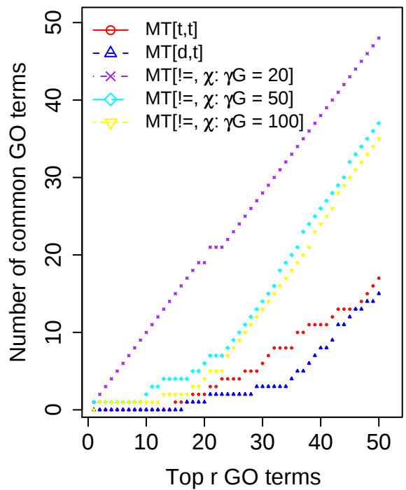
MF, Baseline MT[!=, \chi: \alpha = 0.05 ]
