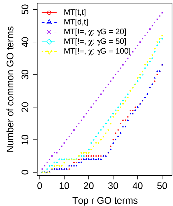
CC, Baseline MT[!=, \chi: \alpha = 0.05 ]
