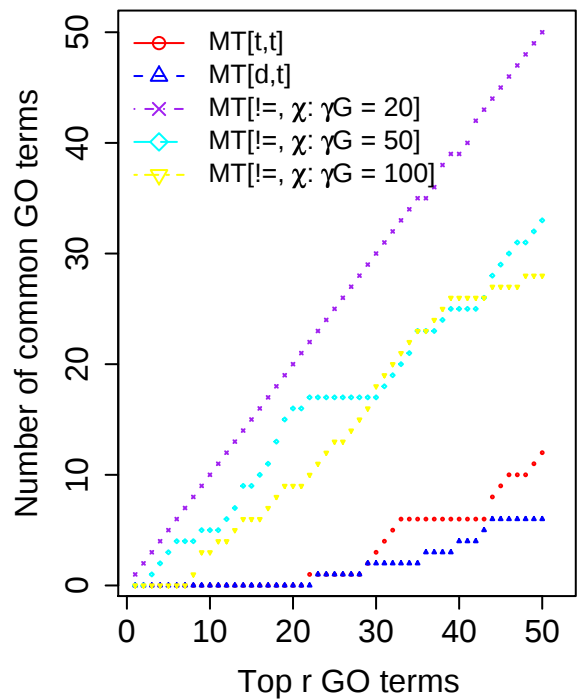
BP, Baseline MT[!=, \chi: \alpha = 0.05 ]
