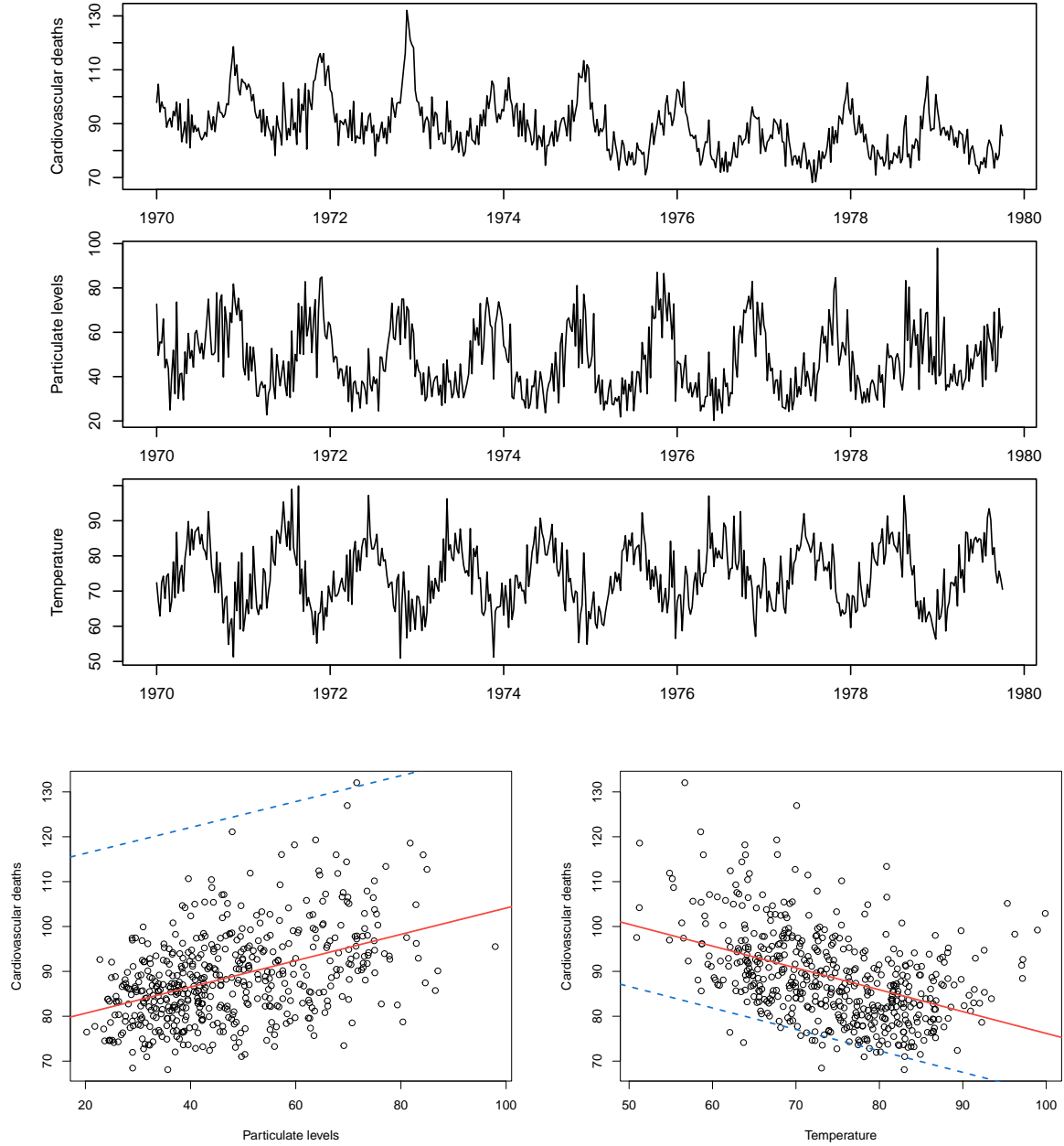
Figure 3: Linear regression of cardiovascular mortality on particulate levels and temperature (this is multiple regression, with two features) in Los Angeles (from SS). The solid red lines denote the estimates from marginal regression; the dashed blue from multiple regression.
