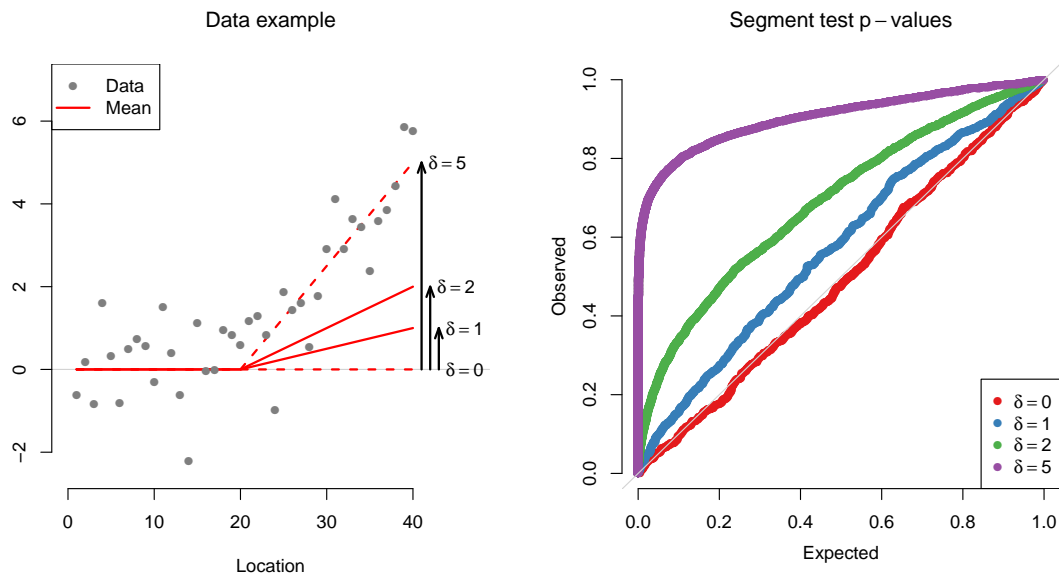
Figure 11: Inferences from the segment test, in a setup with n = 40 points, and one knot in the underlying piecewise linear mean at location 20, with the change in slope is \delta/20 . We considered the settings \delta = 0, 1, 2, 5 . The left panel displays an example simulated data set from this setup, for \delta = 5 . The right panel shows QQ plots of segment test p-values at location 20, computed from the trend filtering path, stopped by the 2-rise BIC rule. The p-values were restricted to repetitions in which location 20 appeared in the BIC-selected model. When \delta = 0 , we see uniform p-values, as appropriate; when \delta = 5 , we see nearly full power.
