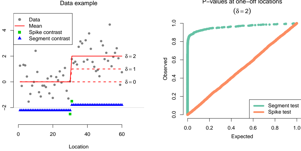
Figure 15: The left panel is copied from Figure 8 in the main text, and shows an example data set with n = 60 and a piecewise constant mean \theta with one jump at location 30. The right panel shows QQ plots from the spike and segment tests run at the detected changepoint from the 1-step fused lasso, over data instances in which the detected changepoint occurred at location 29 or 30, i.e., off by one from the true location 30. We can see that the spike test p-values are uniform, and the segment test p-values are highly sub-uniform.
