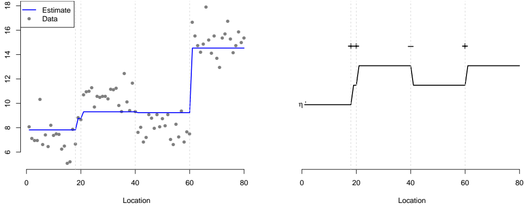
Figure 7: An example showing a 1d fused lasso solution after 4 steps, in the left panel, and its corresponding step-sign plot, in the right panel. Based on the step-sign plot, the data analyst may, e.g., deem locations 18 and 20 to be too close to be both interesting, and merge them before conducting segment tests.
