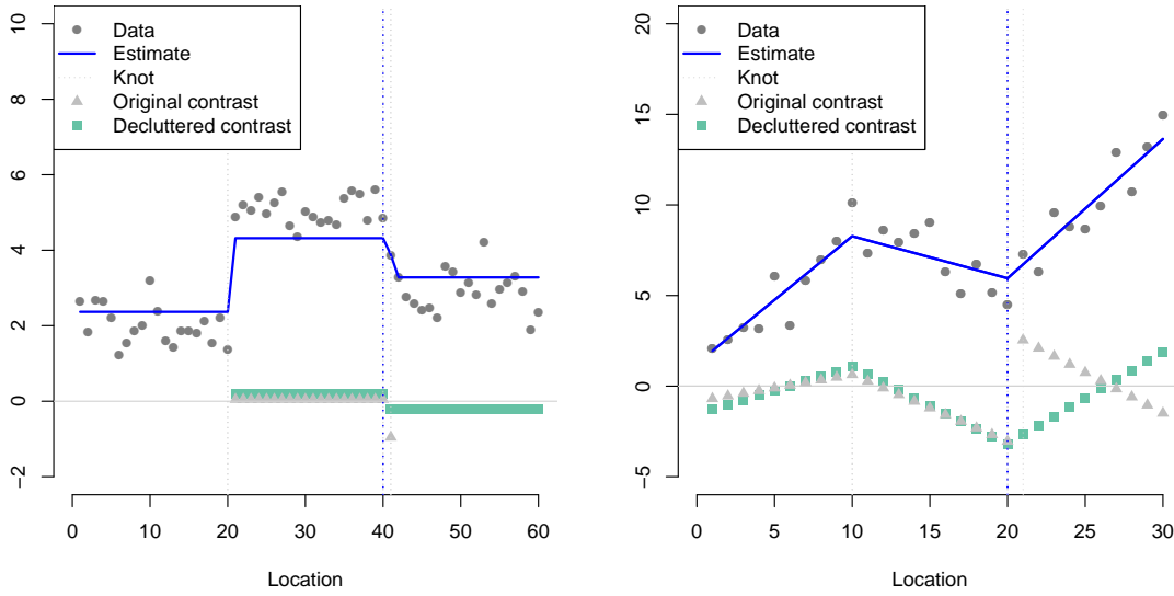
Figure 6: Examples showing the segment test contrasts before and after post-processing or “decluttering” for the 1d fused lasso, in the left panel, and trend filtering, in the right panel. In both problems, the p -values for testing at locations marked by blue dashed vertical lines dropped considerably; on the left, the p -value dropped from 0.236 to <0.001 , and on the right, from 0.09 to 0.001. For trend filtering, it can also be demonstrated that decluttering at one location helps the power for testing at another location that is farther away, but this phenomenon is absent in the fused lasso case (due to the finite support of the segment test contrasts).
