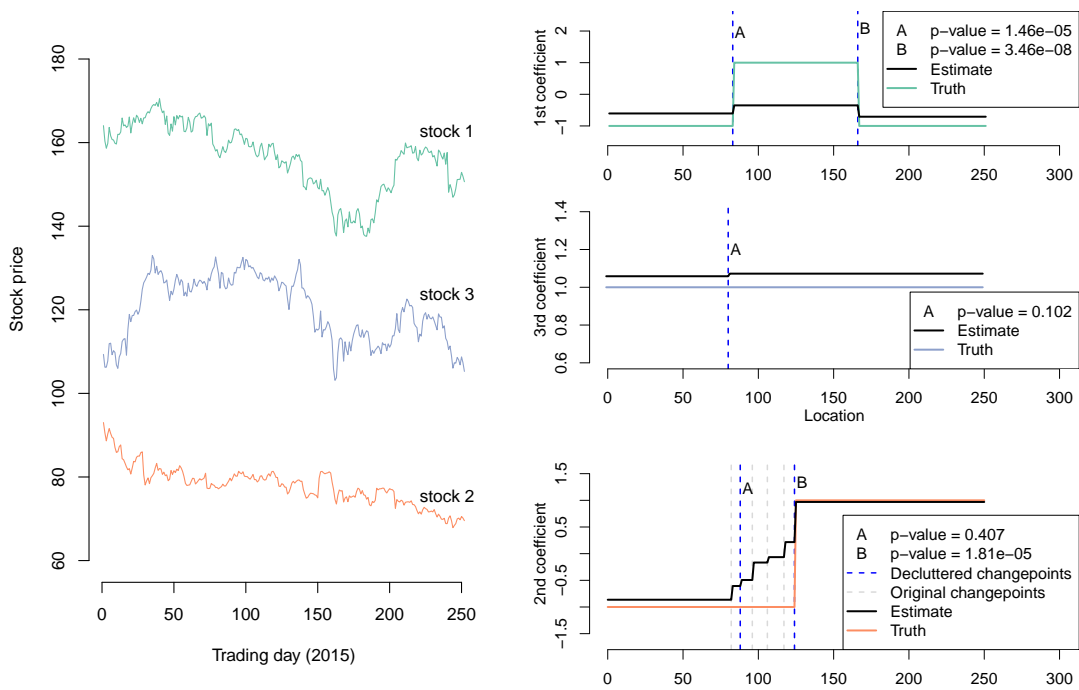
Figure 13: A semi-synthetic stock example, with n = 251 timepoints or trading days. The left panel shows raw stock prices from three DJIA stocks; response data were generated according to a linear model with the log daily returns of these stocks as predictors, and time-varying coefficients. The true piecewise constant time-varying coefficients are displayed in the right panel. The fused lasso regression path was run, and stopped by the 2-rise BIC rule, delivering the estimated coefficients also displayed in the right panel. After decluttering, segment tests were applied to the detected change points and 3 approximately correct locations are deemed significant, with the other 2 spurious detections deemed insignificant.
