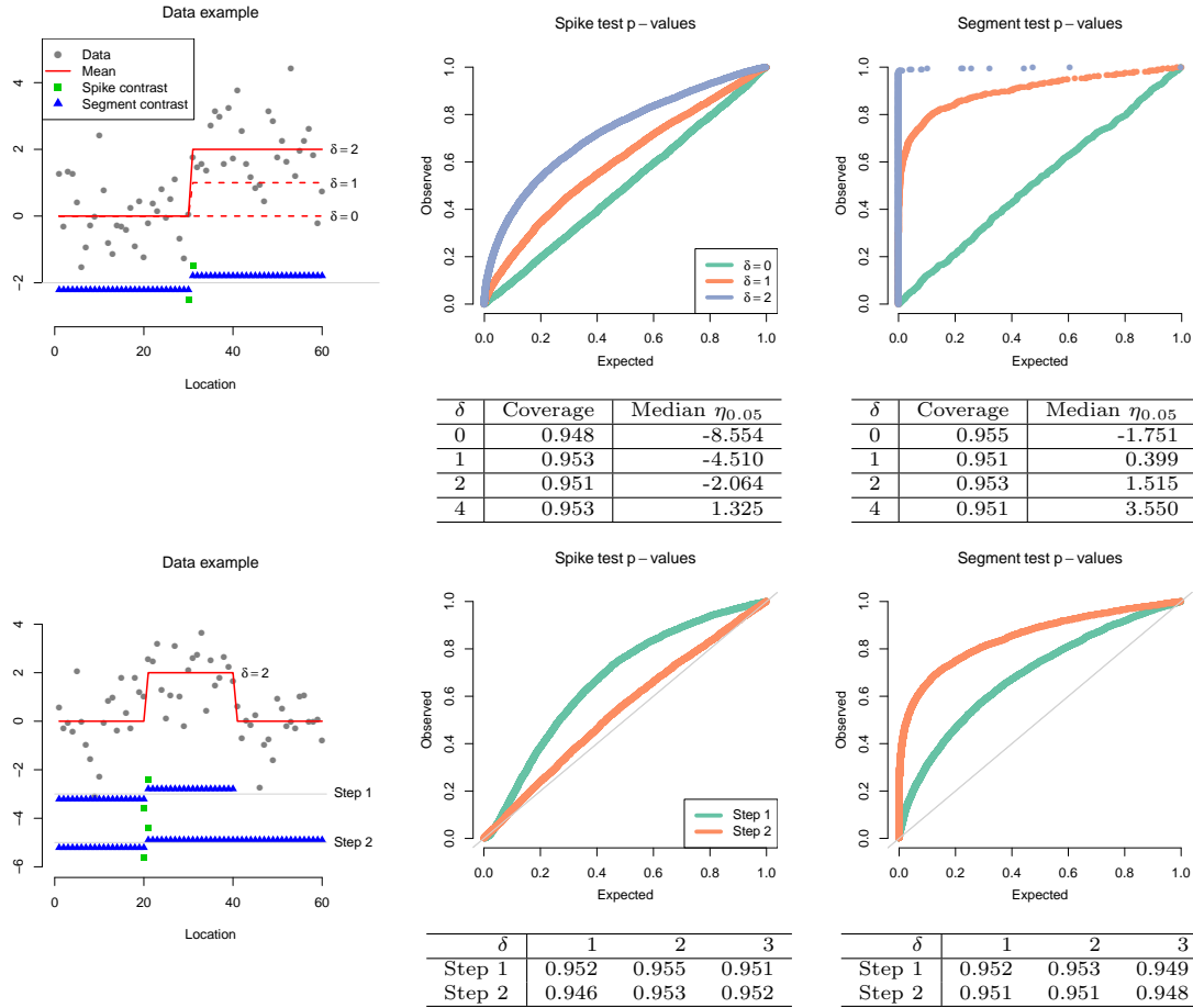
Figure 8: Examination of p -values and confidence intervals coming from the spike and segment tests, in the one-jump (top row) and two-jump (bottom row) settings, with n = 60 points in each case. In the one-jump setting, we considered three signal strengths: \delta = 0, 1, 2 . The top left panel shows an example simulated data set from a one-jump signal with height \delta = 2 , and the middle and right panels show the p -values from the spike and segment tests, collected over simulations for which the 1-step fused lasso correctly detected a changepoint at location 30. We see that the segment test has uniformly higher power. The tables below the plots report empirical coverages of one-sided 95% confidence intervals of the form [\eta_{0.05}, \infty) , along with the median lower bounds \eta_{0.05} . The lower bounds from the segment test are greater than the corresponding lower bounds from the spike test.
