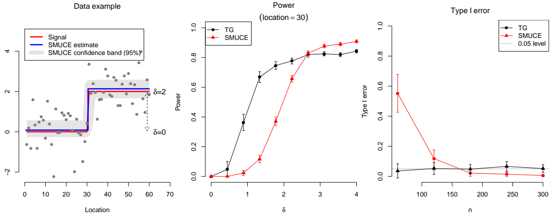
Figure 10: Comparison of p -values from the TG test, and derived from the SMUCE simultaneous confidence band, for testing the same null hypothesis. Data were generated under a problem setup that is the same as that in the top left panel of Figure 8, but with the signal strength \delta varying between 0 and 4. The top left panel of the current figure shows an example with \delta = 2 . In each simulation, the 1d fused lasso path was stopped using the 2-rise BIC rule, and segment test contrasts were formed around the detected changepoints. The middle panel shows power curves, computed over simulations in which the location 30 appeared in the model selected by BIC. These power curves were computed either from the SMUCE band having nominal confidence level 0.95, or the TG test with a type I error control of 0.05. We can see that the latter method has better power for smaller \delta , and both perform well for larger \delta , with the SMUCE-based method providing slightly more power. The right panel displays the empirical type I error of the two testing methods, which emphasizes that the SMUCE guarantees are only asymptotic, and this method can quite become conservative for large n , because in a way simultaneous coverage is a more ambitious goal than post-selection coverage.
