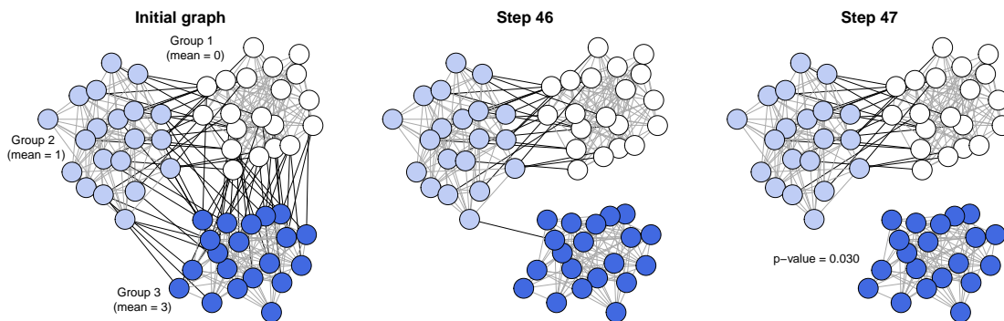
Figure 5: An example with n = 60 nodes illustrating the segment test for the graph fused lasso. The graph was generated using a simple stochastic block model with 3 groups of 20 nodes each. The edge probabilities were 0.5 for nodes in the same group and 0.05 for nodes in different groups. This resulted in m = 369 edges. The group means were defined to be 0, 1, and 3 (colored in white, light blue, and dark blue, above). Data were generated by adding i.i.d. centered Gaussian noise, with standard deviation 0.15. The left plot displays the initial graph, with 321 total edges. The middle plot displays the graph fused lasso estimate after 46 path steps, where there is only one edge left separating group 3 from groups 1 and 2. At step 47, in the right plot, this last edge is removed and the segment test (41), (42) is applied, with C_a being the union of groups 1 and 2 (white and light blue) and C_b being group 3 (dark blue). The p -value is small, around 0.03.
