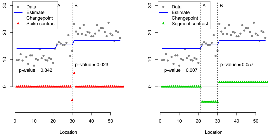
Figure 3: An example with n = 60 points, showing the differences between the spike and segment tests for the fused lasso. The underlying mean has changepoints at locations 20 and 30; the 2-step fused lasso estimate, drawn in blue, detects changepoints at locations 21 and 30, labeled A and B. P-values from the spike test run on both locations are shown in the left panel, and from the segment test in the right panel. The segment and spike contrast vectors corresponding to the test statistic at location B are visualized on the panels (the entries of these vectors have been scaled up for visibility). We can see that both segment p-values are small, and both segment null hypotheses defined around locations A and B should be rejected; but only the spike p-value at location B is small, and only the spike null hypothesis around location B should be rejected (as location A does not correspond to a true changepoint in the underlying mean, it is one position larger than the first true changepoint).
