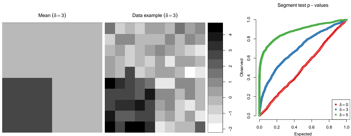
Figure 12: Inferences from the segment test, in a 2d problem setup with n = 100 , and a mean parameter \theta shaped into a piecewise constant 10 \times 10 image. The bottom 5 \times 5 block of the mean is assigned a height of \delta , and the rest of its components 0. We considered the settings \delta = 0, 3, 5 . The left panel visualizes the mean \theta , when \delta = 3 ; the middle panel shows an example noisy realization y , again for \delta = 3 . The right panel shows QQ plots of the segment test, with respect to two fused components appearing in the 2d fused lasso estimate, stopped by the 1-rise BIC stopping rule. When \delta = 3, 5 these p-values are restricted to data instances in which the components being tested are the lower left 5 \times 5 block and its complement; when \delta = 0 , all p-values are shown. The p-values behave as we would expect: uniform for \delta = 0 , and increasing power for \delta = 3, 5 .
