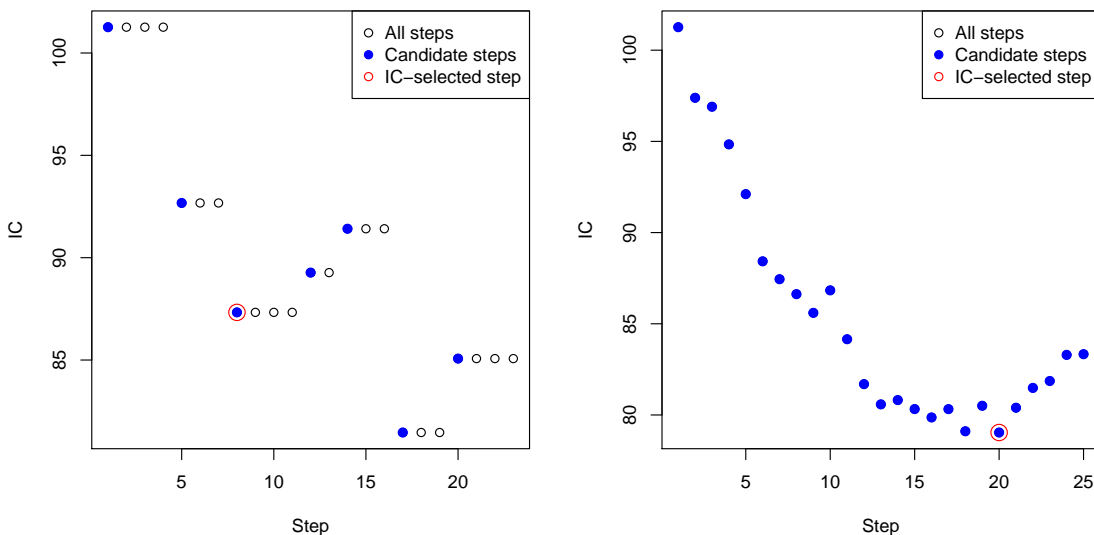
Figure 2: Two illustrations of the IC selection rule with q = 2 ; on the left, an example where \text{null}(D_{-\mathcal{B}_k}) changes at just 6 steps (representing, e.g., the 2d fused lasso case); on the right, an example where \text{null}(D_{-\mathcal{B}_k}) changes at every step (representing, e.g., the 1d fused lasso case). In both panels, solid blue circles mark the candidate set \hat{I}^{\text{C}}(y) in (15), and a large red circle is drawn around the IC-selected step in (16).
