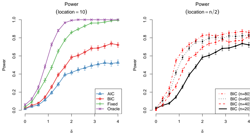
Figure 9: Power curves for a one-jump signal with n = 20 points on the left, and n = 20, 40, 60, 80 on the right, and in each case, having a jump at location n/2 , of height \delta . The left panel shows the results from the segment test, either at step 1 (labeled “Fixed”, in green), or at a step selected by the 2-rise AIC or BIC rule (labeled “AIC” and “BIC”, in blue and red, respectively). The power curves were computed from p-values over simulations in which location 10 appeared in the selected model (and the AIC- and BIC-based rules applied appropriate corrections for multiplicity). The left panel also shows the results of applying an oracle test at location 10, for equality of means. We can see a clear drop in power from the oracle to the fixed rule to the IC-based rules. The right panel shows the improvement in BIC power curves as n increases.
