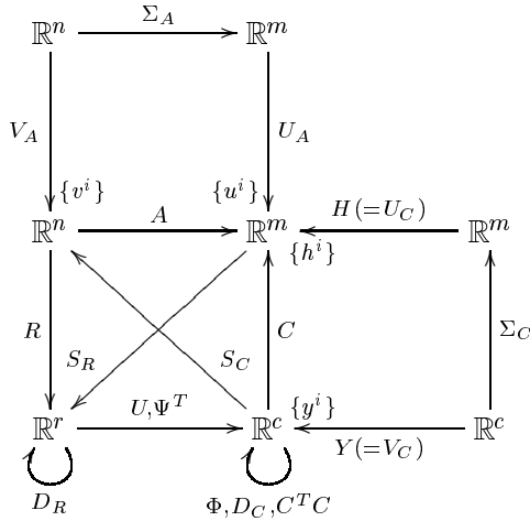
Figure 4: Another diagram for the LINEARTIMECUR Algorithm
