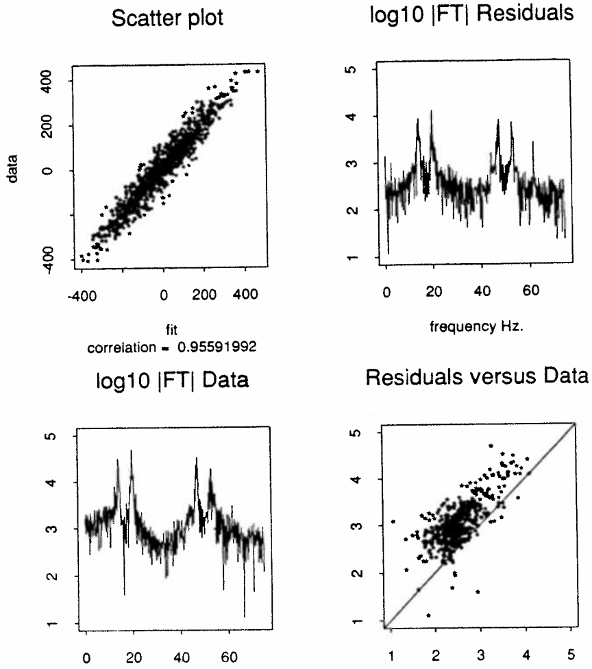
FIGURE 12 - THIRD 1000 POINTS
