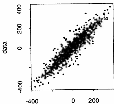
Scatter plot
