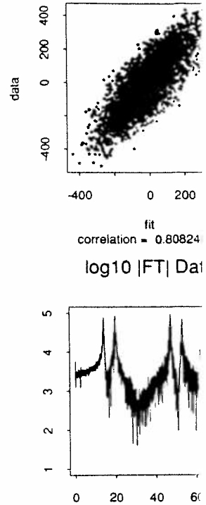
FIGURE 9 - Scatter plot
