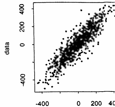
Scatter plot
