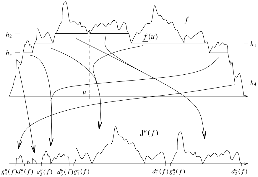
Fig. 1. The Joyal functional, with three strictly generalized excursions
