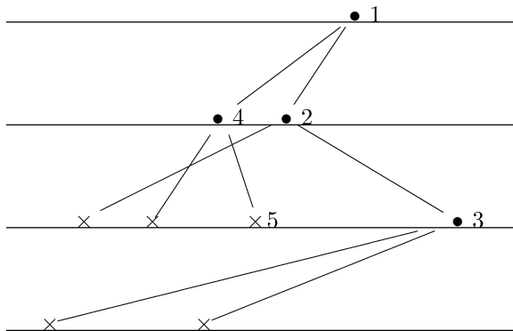
FIG. 3. Algorithmic exploration of BRW. The individuals \bullet have been queried in order 1, 2, 3, 4; the children \times have not yet been queried. Individual 5 will be queried next.
