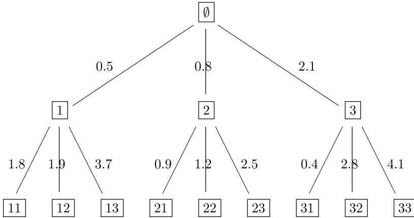
FIG. 4. Part of a realization of the PWIT that shows just the first three children of each vertex. The length is written next to each edge e .
