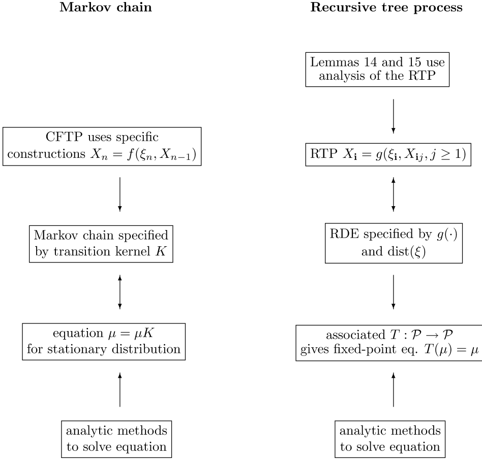
FIG. 2. The analogy between Markov chains and RTPs. Specifying a transition kernel is exactly what is needed to write the equation for a stationary distribution, and exactly what is needed to specify the chain. Analogously, specifying S and g(\cdot) and \text{dist}(\xi) is exactly what is needed to write the RDE, and exactly what is needed to specify the RTP. But note these equivalences \Downarrow occur at different conceptual levels.
