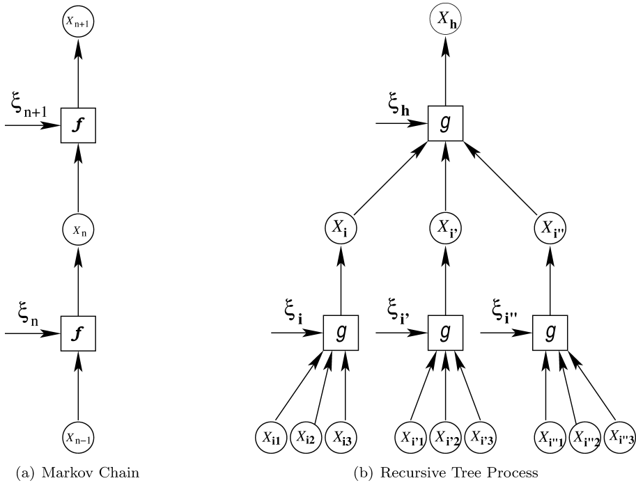
FIG. 1. On the left is a Markov chain represented as an iterated function system: X_n is the “output” of f with “inputs” \xi_n and X_{n-1} . On the right is an RTP; X_{\mathbf{i}} is the “output” of g with inputs \xi_{\mathbf{i}} and (X_{\mathbf{j}}, \mathbf{j} child of \mathbf{i} ). In the figure, \mathbf{h} is the parent of \mathbf{i} and \mathbf{i}', \mathbf{i}'', \dots are siblings of \mathbf{i} .
