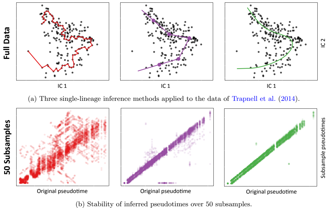
Figure 2: Pseudotime inference: Robustness to noise . We examine the stability of three lineage inference methods, showing how each method orders the cells for the original dataset as well as for 50 subsamples of the data. Panel (a) : Monocle identifies the longest path through the MST constructed on all cells (red). Waterfall and TSCAN cluster cells and connect cluster centers with an MST (purple, clustering performed by k -means with k = 5 ). A principal curve is a non-linear fit through the data, used by Embeddr and Slingshot (green). As in Trapnell et al. (2014) , dimensionality reduction is performed by ICA. Panel (b) : We examine the stability of these three methods by plotting pseudotimes based on 50 subsamples of the data vs. the original pseudotimes. Subsamples were generated in a bootstrap-like manner, by randomly sampling n times with replacement from the original cell-level data and retaining only one instance of each cell. Thus, subsamples were of variable sizes, but contained on average about 63% of the original data. The cluster-based MST method occasionally detected spurious branching events and, for the purposes of visualization, cells not placed along the main lineage were assigned a pseudotime value of 0.
