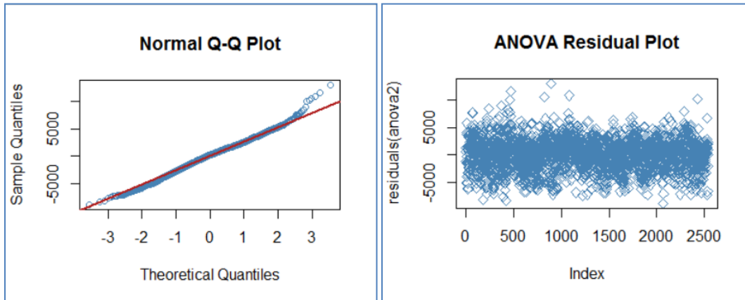
Figure 4: QQ and Scatter Plot of ANOVA Residuals
