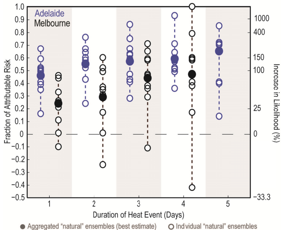
FIGURE 4.2 The single very hot days in Melbourne still show a large spread in FAR values despite the higher frequency of such events under both the “natural” and “all forcings” climate scenarios, compared with the counterfactual. This figure shows FAR and the corresponding increase in likelihood calculated for Adelaide (blue) and Melbourne (black) heat waves of different durations. The temperature threshold used to define heat waves was 42°C for Adelaide and 41°C for Melbourne. Ten “natural” ensembles are aggregated (black symbols) in order to calculate a best estimate of FAR, while each of the “natural” ensembles is considered separately (white symbols) in order to better sample the possible range of FAR values and estimate uncertainties. SOURCE: Black et al., 2015.
