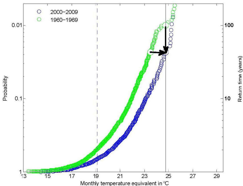
FIGURE S.2 Western Russia experienced several heat waves in summer 2010, leading to average temperatures in July 2010 exceeding the long-term observed average by more than 5°C. This extreme heat prompted questions about the potential effect of human-caused climate change. To address this question, Otto et al. (2012) use an atmospheric general circulation model to produce hundreds of simulations of the climate of the 2000s (blue circles) and of the 1960s (green circles). Defining heat waves as having high temperatures and anti-cyclonic circulation anomaly (associated with persistent conditions), they examined how likely it would be for temperature to exceed a given magnitude. Using this approach, the authors concluded that the average observed temperature during July 2010 of nearly 25°C was significantly more likely in the 2000s than in the 1960s, corresponding to a shift from a 99-year return time to a 33-year return time (downward black arrow; horizontal arrow explained in Figure 2.1). SOURCE: Figure courtesy of Friederike Otto, adapted from Otto et al. (2012).
