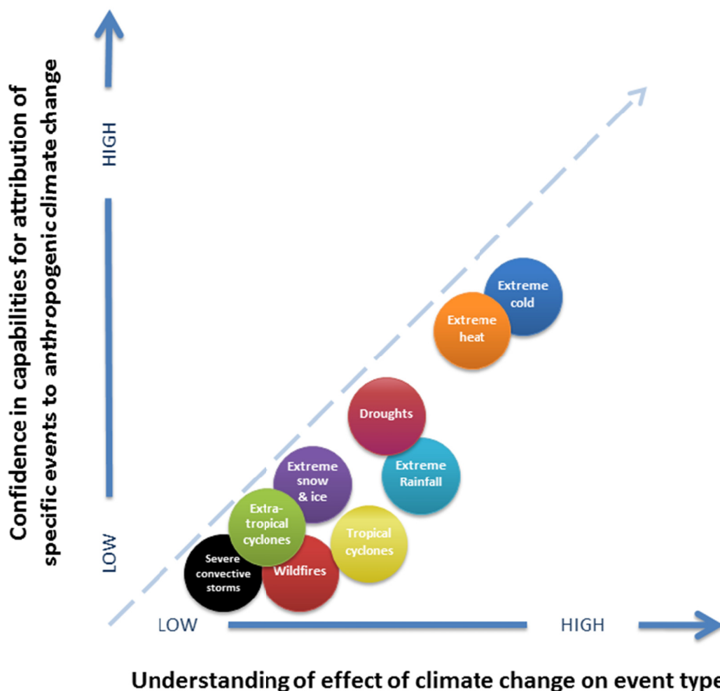
FIGURE S.4 Schematic depiction of this report’s assessment of the state of attribution science for different event types. The horizontal position of each event type reflects an assessment of the level of understanding of the effect of climate change on the event type, and corresponds to the right-most column of Table S.1. The vertical position of each event type indicates an assessment of scientific confidence in current capabilities for attribution of specific events to anthropogenic climate change for that event type, and draws upon all three columns of Table S.1. A position below the 1:1 line indicates an assessment that there is potential for improvement in attribution capability through technical progress alone (such as improved modeling, or the recovery of additional historical data), which would move the symbol upward. A position above the 1:1 line is not possible because this would indicate confident attribution in the absence of adequate understanding. In all cases, there is potential to increase event attribution confidence by overcoming remaining challenges that limit the current level of understanding. See Box 4.1 for more detail.
