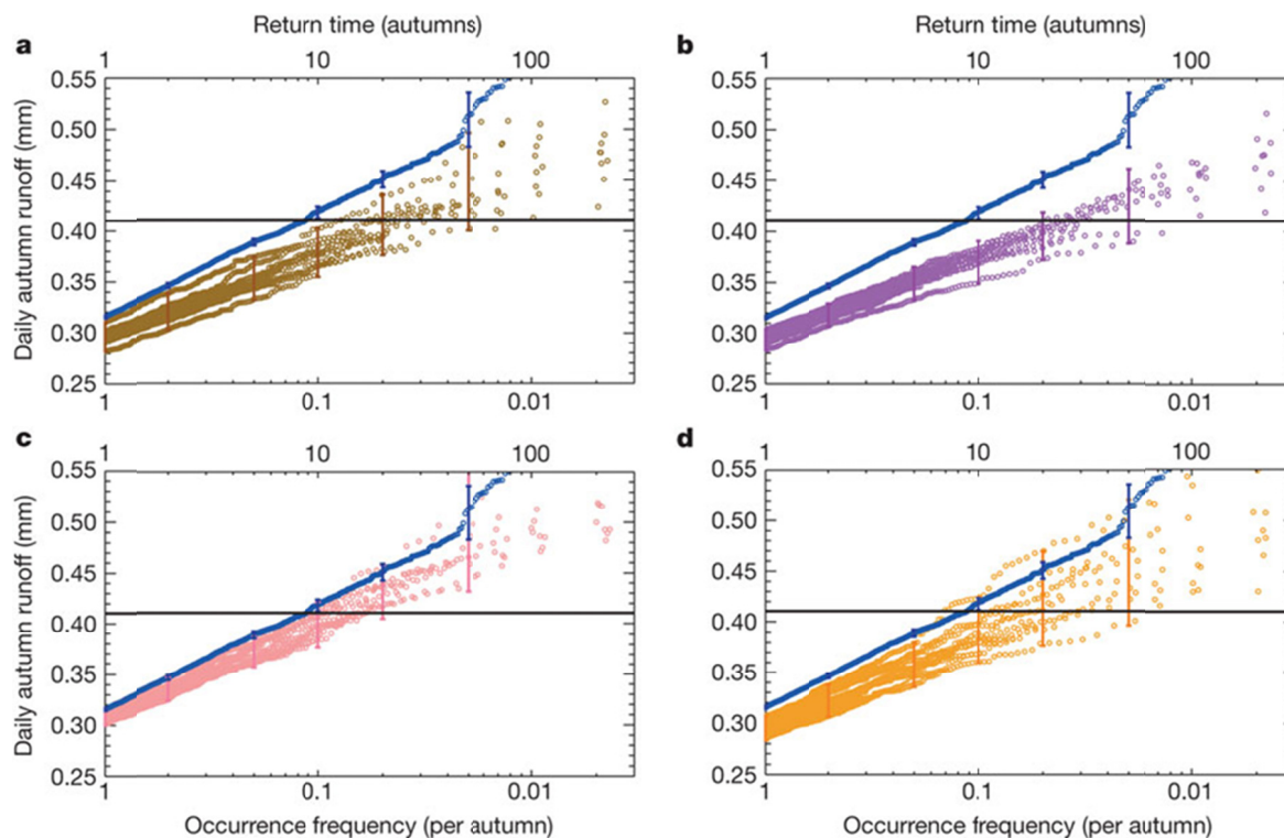
FIGURE 3.4 Sensitivity of change in the occurrence frequency of extremely high river runoff in England and Wales for autumn 2000 using different climate models to characterize and remove the human influence on sea surface temperature from a counterfactual world. This figure illustrates that while present condition runoff return periods tend to be more frequent than those in any such counterfactual world, the occurrence frequencies in a counterfactual world depend on the model used to create it. Blue is the modeled return time for 2000 runoff (identical in each panel) against occurrence frequency, while colored dots show the return times in a counterfactual world, constructed by removing the pattern of human influence on SSTs from four different climate models: HadCM3 (brown, a), GFDL (purple, b), PCM (pink, c) and MIROC (orange, d). The horizontal black line on each panel corresponds to the highest daily runoff observed during these two months. SOURCE: Pall et al., 2011.
