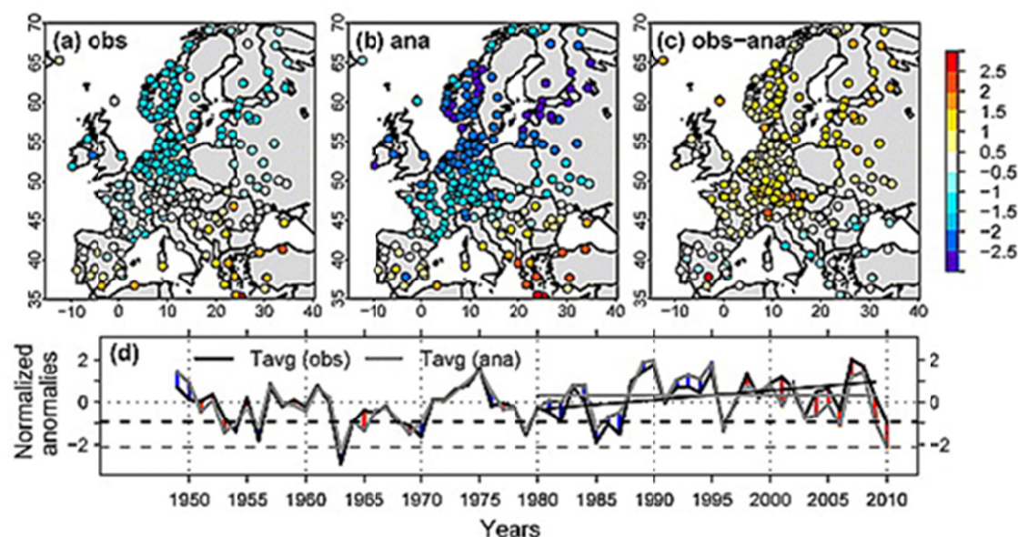
FIGURE 3.3 Example of an analysis using observational circulation analogues, investigating the unusually cold winter conditions in Europe in 2010. In the top figure, panel (a) shows observations of winter 2010 European temperatures; panel (b) shows an average of winters with similar daily circulation over the 2nd half of the 20th century (analog); and panel (c) shows the difference between both. The time series (bottom figure) analyzes the (averaged over all European stations) winter 2010 anomaly of daily mean temperature of -1.3^{\circ}\text{C} (indicated by a dashed line) in the context of the historical record and analogues. It shows normalized 1949–2010 time series of observed (black line) and analog mean temperature anomalies (gray line), illustrating the warming of observed winters relative to analogue winters (red segments: positive observed–analog differences, blue segments: negative observed–analog differences). SOURCE Cattiaux et al., 2010.
