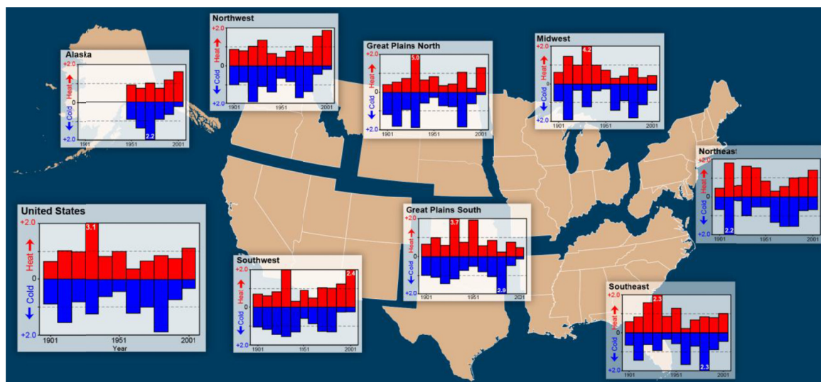
FIGURE 3.5 Time series of decadal average values of heat wave (red bars) and cold wave (blue bars) indices over various regions of the United States; the average for the entire United States is shown at the lower left. These indices are a normalized (to an average value of 1.0) metric of the number of extreme temperature events for spells of 4-day duration. An event is considered extreme if the average temperature exceeds the threshold for a 1-in-5 year recurrence. The horizontal labels give the beginning year of the decade. Recent decades tend to show an increase in the number of heat waves and a decrease in the number of cold waves but over the long-term, the drought years of the 1930s stand out as having the most heat waves. SOURCE: Peterson et al., 2013a.
