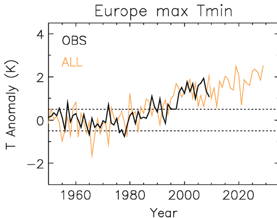
FIGURE 4.1 This figure shows a time series of the annual maximum nighttime temperature averaged over the European Region. Temperatures are plotted as anomalies, or deviations from normal (in this case, 1961-1990), in degree Kelvin (K). Observed temperatures are represented by the black lines (OBS) and are based on Caesar et al. (2006; updated). The orange lines (ALL) come from model simulation (Martin et al., 2006). Both observations and model output show an increasing trend in nighttime temperature anomalies over time. The horizontal dotted lines denote the uncertainty range (5-95%) due to natural climate variability. SOURCE: Stott et al., 2011.
