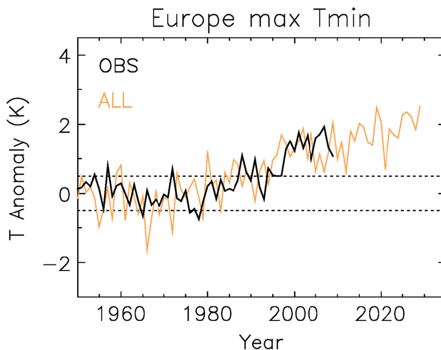
FIGURE S.1 This figure shows a time series of the annual maximum nighttime temperature averaged over the European Region. Temperatures are plotted as anomalies, or deviations from normal (in this case, 1961-1990), in degree Kelvin (K). Observed temperatures are represented by the black lines (OBS) and are based on Caesar et al. (2006; updated). The orange lines (ALL) come from model simulation (Martin et al., 2006). Both observations and model output show an increasing trend in nighttime temperature anomalies over time. The horizontal dotted lines denote the uncertainty range (5-95%) due to natural climate variability. SOURCE: Stott et al., 2011.
