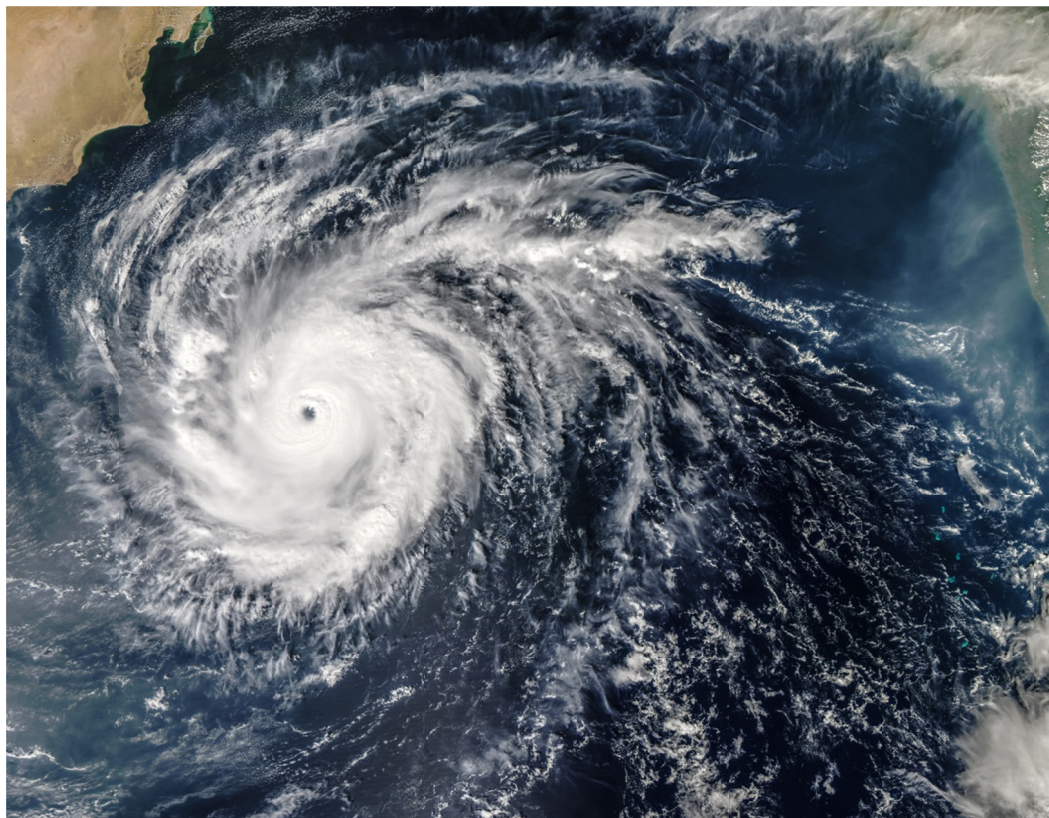
FIGURE 4.6 The Moderate Resolution Imaging Spectroradiometer (MODIS) on NASA's Aqua satellite acquired this image of Cyclone Chapala (04A) approaching the Arabian Peninsula on October 30, 2015 (it made landfall in early November 2015). Only two tropical cyclones have hit the Peninsula since reliable records started in 1979. At the time of this image, the tropical cyclone had sustained winds between 130 and 135 knots (150-155 miles or 240-250 kilometers per hour) and significant wave heights of 38 feet. SOURCE: NASA. http://earthobservatory.nasa.gov/NaturalHazards/view.php?id=86899 .
