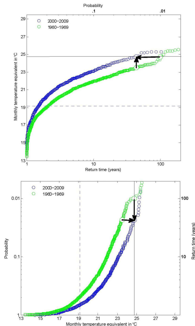
FIGURE 2.1 Different ways of describing the effect of anthropogenic climate change on July heat waves over western Russia, motivated by the extreme heat wave of summer 2010. Heat waves are here defined by a combination of high temperature and anti-cyclonic circulation anomaly (associated with persistent conditions). Both figures show model estimates of the likelihood of occurrence of an extreme of at least the given magnitude for 1960s (green) and 2000s (blue) conditions, expressed either as a return time or as a probability. The top figure shows magnitude versus probability (or return time), whereas the bottom figure shows the same data plotted as probability (or return time) versus magnitude, which is related to the cumulative distribution function commonly encountered in statistics but here shows probability of exceedance rather than the usual probability of non-exceedance. In both panels the magnitude of the July 2010 Russian heat wave (indicated by the thin black line) corresponds to a large change in likelihood arising from climate change (from a 99-year return time to a 33-year return time, indicated by the horizontal arrow in the top figure and the vertical arrow in the bottom figure), but to a small (compared to the overall anomaly of 2010 with respect to average July conditions (dashed line)) relative change in magnitude (indicated by the vertical arrow in the top figure and the horizontal arrow in the bottom figure). SOURCE: Figure courtesy of Friederike Otto, adapted from Otto et al. (2012).
