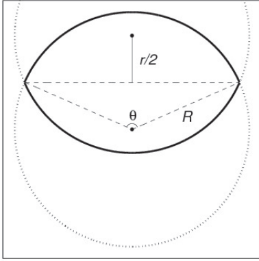
FIG. 40 The overlap between the two disks (area comprised within the bold line) gives the quantity \rho_2(r) . From [104].
