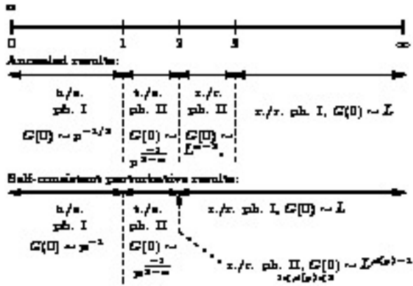
FIG. 71 Phase diagram for d = 1 . The annealed approximation shows some differences with the self-consistent approximation for the quenched case. In the quenched case, the walk is transient for \alpha < 2 and recurrent for \alpha \geq 2 . From [198].
