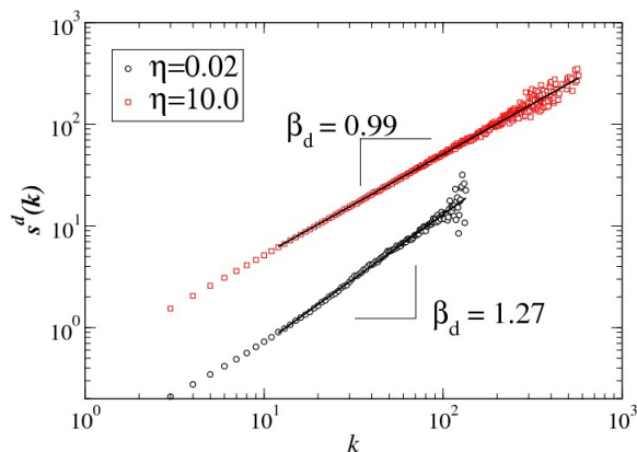
FIG. 47 Distance strength versus k for two different cases ( \eta = 0.02 and \eta = 10.0 ). When \eta is not small, space is irrelevant and there are no correlations between degree and space as signalled by \beta_d \approx 1 . When spatial effects are important ( \eta = 0.02 \ll 1 ), non-linear correlations appear and \beta_d > 1 . We observe a crossover for k \simeq 10 - 20 to a power-law behavior and the power-law fit over this range of values of k is shown (full lines). From [31].
