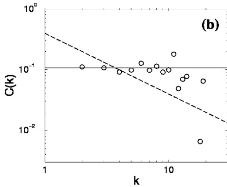
FIG. 28 Scaling of the clustering C(k) for the Power Grid of the Western United States. The dashed line has a slope -1 and the solid line corresponds to the average clustering coefficient. From [263].
