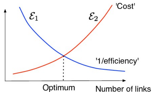
FIG. 63 Schematic representation of many optimal network models. The functional to minimize is the sum of two terms which behave in opposite way when adding links. This leads in general to a non-trivial optimum.
