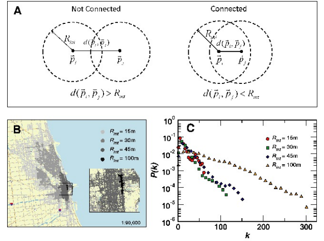
FIG. 85 (a) Construction of the WIFI network as a random geometric graph (see section IV.A.1). (b) Giant component of the WIFI network in Chicago for different values R_{int} . (c) Degree distribution for different values of R_{int} . From [164].
