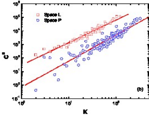
FIG. 17 Betweenness centrality versus the degree k . The power law fit for the L-space gives 1.66 and 1.93 in the P-space. From [165].
