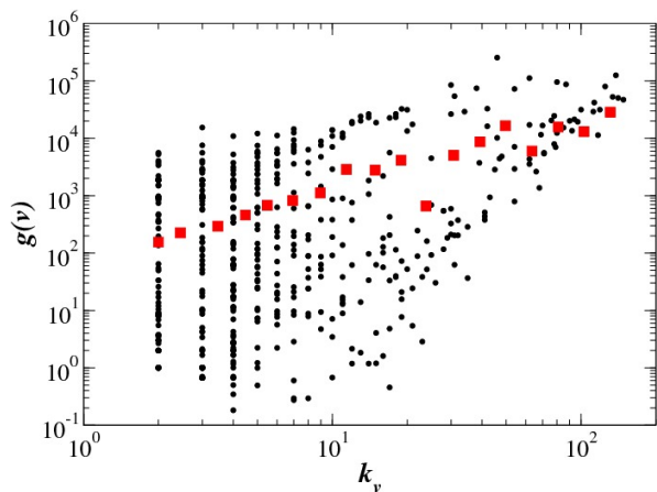
FIG. 10 Scatter-plot of the betweenness centrality versus degree for nodes of the North American air-transportation network. The (red) squares correspond to the average betweenness centrality versus degree. From [31].
