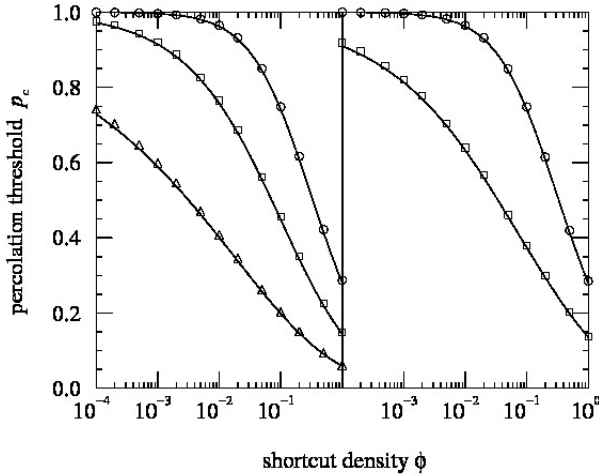
FIG. 76 Numerical solution for the percolation threshold for N = 10^6 for site and bond percolation (shown left and right, respectively). Circles represent the case k = 1 , squares k = 2 , and triangles k = 5 . From [236].
