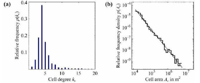
FIG. 22 (a) Degree distribution of degrees for the road network of Dresden. (b) The frequency distribution of the cells surface areas A_c obeys a power law with exponent \alpha \approx 1.9 (for the road network of Dresden). From [206].
