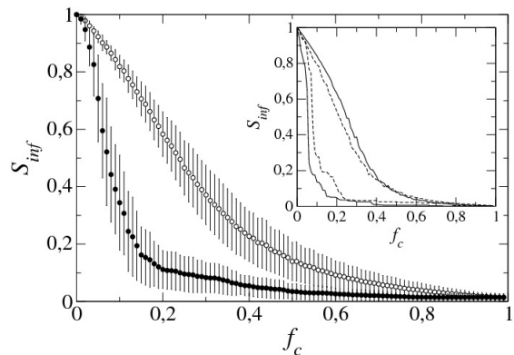
FIG. 78 Effect of random removal of nodes (white circles) and targeted attacks (black circles) on the relative size of the largest component of the EU power grid. In the inset, the effect of random removal and targeted attacks are shown for Italy (dashed lines) and France (continuous line). From [288].
