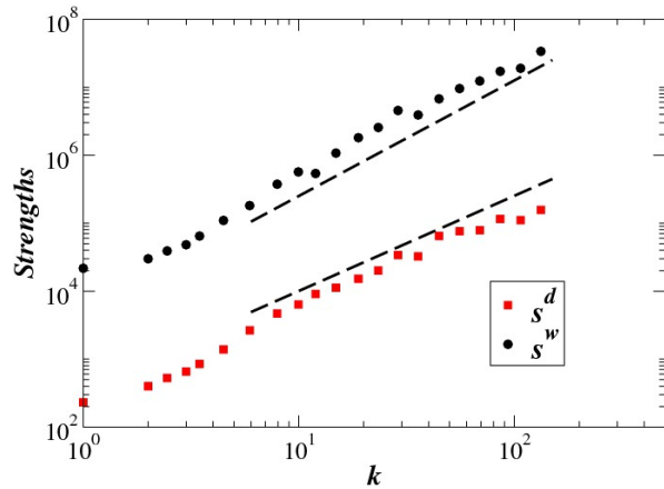
FIG. 8 Weight and distance strengths versus degree for the North American network. The dashed lines correspond to the power-laws with exponents \beta_d \simeq 1.4 and \beta_w \simeq 1.7 . From [31].
