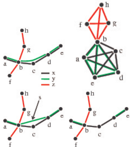
FIG. 6 (a) Direct representation of the routes (here for three different routes). (b) Space-of-changes (sometimes called P space [207, 283, 286]). A link connects two nodes if there is at least one vehicle that stops at both nodes. (c) Space-of-stops. Two nodes are connected if they are consecutive stops of at least one vehicle. (d) Space-of-stations. Here two stations are connected only if they are physically connected (without any station in between) and this network reflects the real physical network. From [203].
