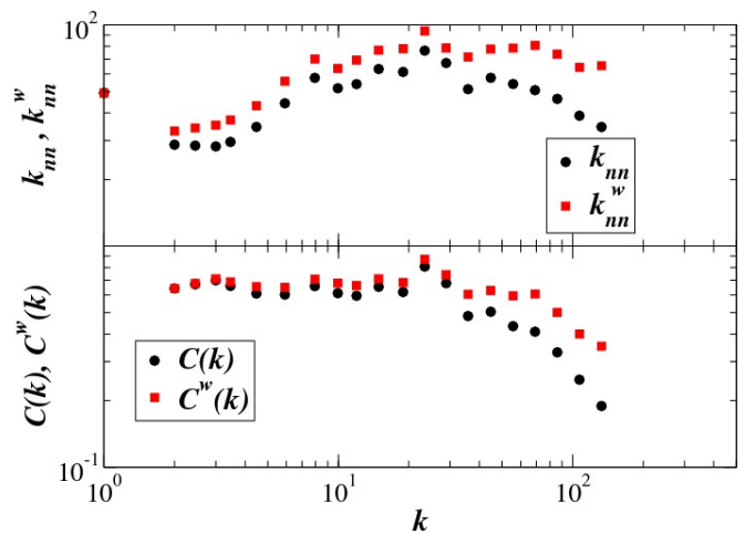
FIG. 9 Assortativity and clustering for the North American network. Circles correspond to topological quantities while the squares represent the weighted assortativity and clustering. From [31].
