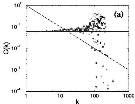
FIG. 30 Scaling of the clustering C(k) for the Internet at the router level. The dashed line has a slope -1 and the solid line corresponds to the average clustering coefficient. From [263].
