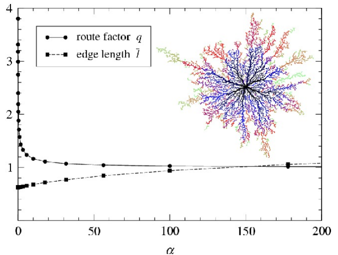
FIG. 50 Route factor q and average edge length \bar{l} versus \alpha in Eq. (175). These results are obtained for N = 10^4 vertices and in the inset the network is obtained for \alpha = 12 . From [135].
