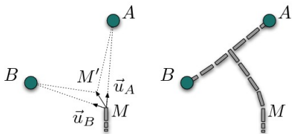
FIG. 51 M is the closest network's point to both centers A and B . The road will grow to point M' in order to maximally reduce the cumulative distance \Delta of A and B from the network. From [39].
