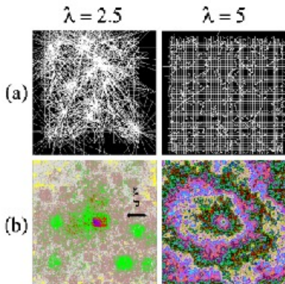
FIG. 41 Spatial structure of the network obtained by the method proposed in [271] for different values of the exponent \lambda of degree distribution. In (a) the networks are shown and in (b) the corresponding chemical shells of equidistant sites form the central node. From [271].
