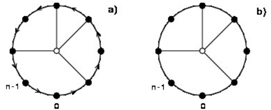
FIG. 58 Models proposed in [112] and studied in [19, 171] with congestion. A central site is connected to a site on a ring with probability p . In (a) all the links on the ring are directed and in (b) these links are not directed. From [112].
