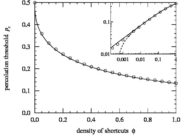
FIG. 77 Percolation threshold for a two-dimensional Watts-Strogatz network with a fraction \phi of shortcuts (the lines are the analytical calculations and the circles represent the numerical simulation). The inset is the zoom in loglog on the small \phi region (the numerical simulation is compared with the analytical calculation for the quantity 1/2 - p_c ). From [249].
