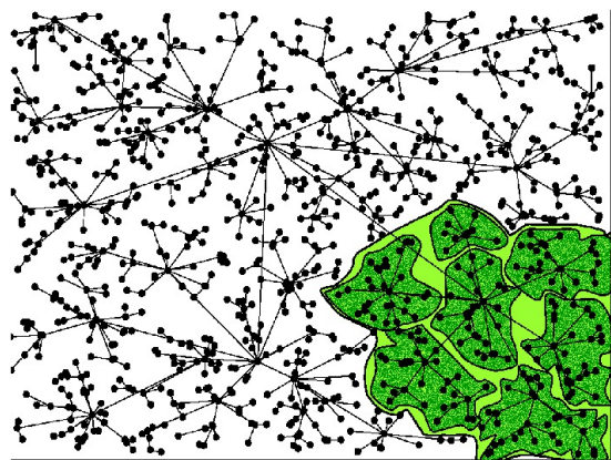
FIG. 61 Hierarchical organization emerging for the optimal traffic tree (\mu, \nu) = (1/2, 1/2) ( N = 10^3 nodes). Longer links lead to regional hubs which in turn connect to smaller hubs distributing traffic in smaller regions. From [38].
