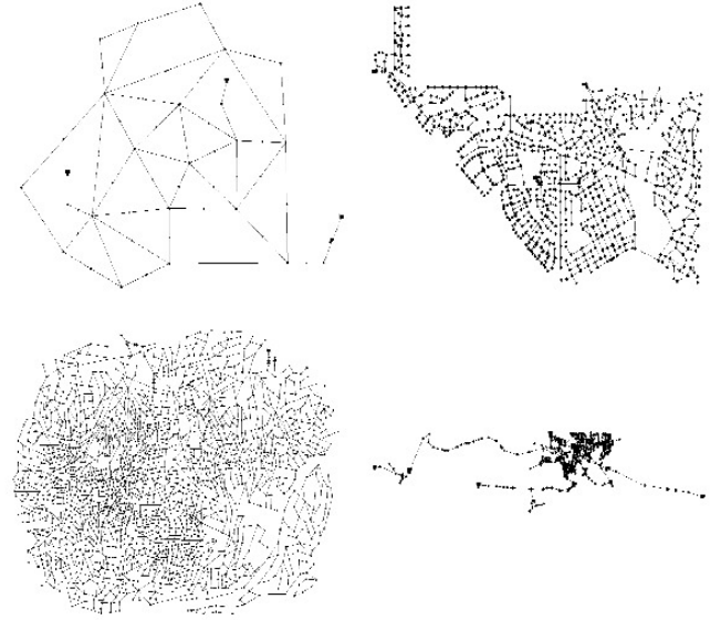
FIG. 29 Representation of water distribution networks. Left panels (from top to bottom): Synthetic networks (‘Anytown’ [307], and ‘EXNET’ [127]). Top-right panel: Colorado Spring Utilities network. Bottom-right panel: Richmond (UK) water distribution network. From [326].
