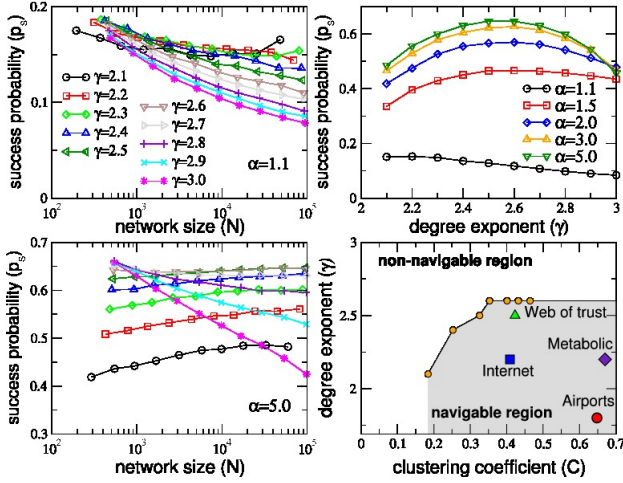
FIG. 75 (a,b) Success probability p_S versus N for various values of \gamma and for (a) weak clustering and (b) strong clustering. (c) Success probability p_S versus \gamma for various values of \alpha and for fixed system size N \approx 10^5 . (d) The solid line separates the navigable from the non-navigable region. From [57].
