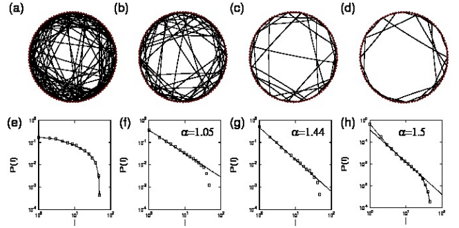
FIG. 67 (a-d) Examples of networks constructed for different values of \lambda = 0.05, 0.3, 0.8, and 0.95 . (e-h) Corresponding link length distribution for these different values of \lambda . Straight lines in (f-h) represent power laws with exponent 1.05, 1.44, and 1.5, respectively. From [62].
