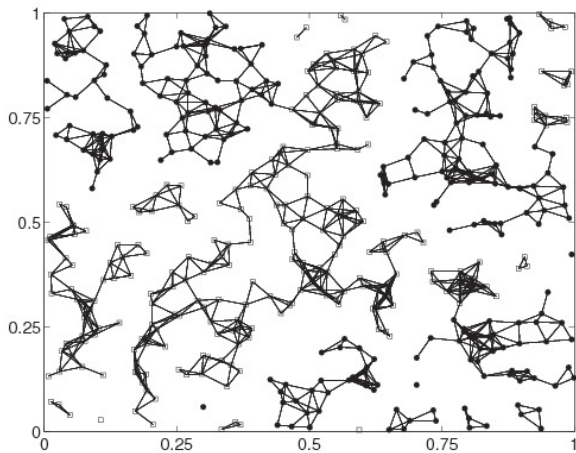
FIG. 39 Example of a 2d random geometric graph obtained for N = 500 spheres and \langle k \rangle = 5 . From [104].
