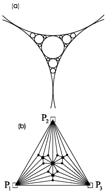
FIG. 42 Top: Classical Apollonian packing. Bottom: Apollonian network (showing the first, second and third generation with circles, squares, dots symbols respectively). From [178].
