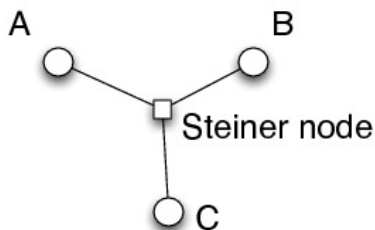
FIG. 62 Example of the Steiner tree for three points A , B , and C . The Steiner point S is located at the Fermat point of the triangle ABC and minimizes the total distance d(S, A) + d(S, B) + d(S, C) . The angles are equal (SB, SA) = (SA, SC) = (SC, SA) = 2\pi/3 .
