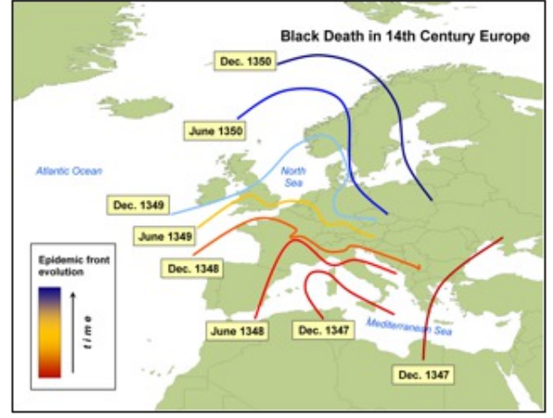
FIG. 81 Spread of the Black Death during the 14th century. The epidemic front spreads in Europe with a velocity of the order of 200400 miles per year. From [94].
