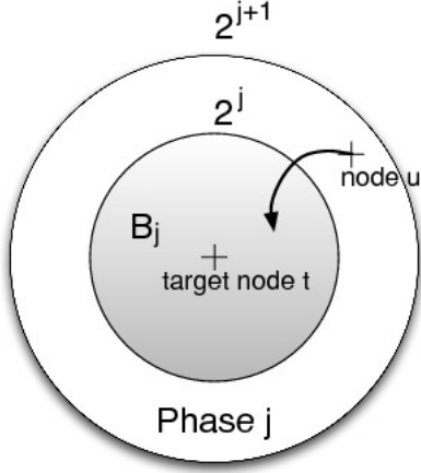
FIG. 73 Line: jump out of the phase j into the domain B_j .
