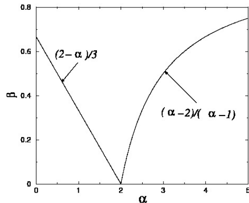
FIG. 72 Lower bounds of the exponent governing the behavior of the average delivery time \bar{T} as a function of the exponent \alpha controlling the distribution of shortcuts. After [195].
