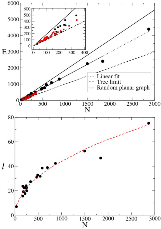
FIG. 20 (a) Numbers of roads versus the number of nodes (ie. intersections and centers) for data from [73] (circles) and from [66] (squares). In the inset, we show a zoom for a small number of nodes. (b) Total length versus the number of nodes. The line is a fit which predicts a growth as \sqrt{N} (data from [73] and figures from [39]).
