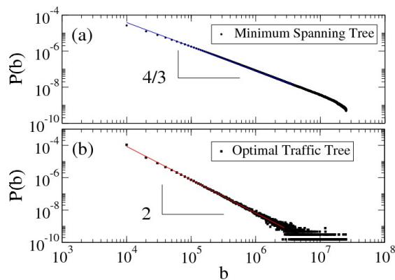
FIG. 60 Betweenness centrality distribution for the MST and for the OTT. The lines are power law fits and give for the MST the theoretical result \delta = 4/3 and for the OTT the value \delta \simeq 2.0 ( N = 10^4 , 100 configurations). From [38].
