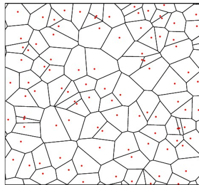
FIG. 2 Example of the Voronoi tessellation on a set of points. From [160].
