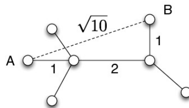
FIG. 5 Example of a detour index calculation. The ‘as crow flies’ distance between the nodes A and B is d_E(A, B) = \sqrt{10} while the route distance over the network is d_R(A, B) = 4 leading to a detour index equal to Q(A, B) = 4/\sqrt{10} \simeq 1.265 .
