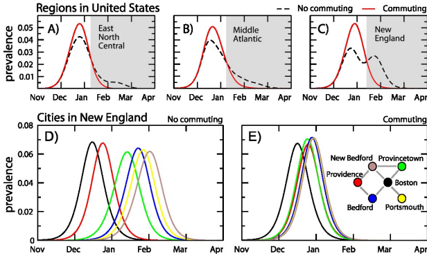
FIG. 84 Comparison of prevalence profiles without and with commuting flows. (a-b-c) Prevalence profiles for three continental US regions. (d-e) Prevalence profiles for cities in New England. From [25].
