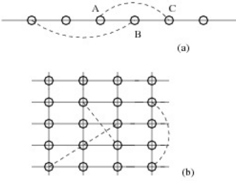
FIG. 45 Schematic representation of spatial small-world in (a) one dimension and (b) two dimensions. The dashed lines represent the long-range links occurring with probability q(\ell) \sim \ell^{-\alpha} . From [282].
