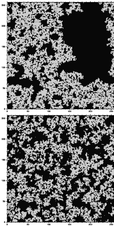
FIG. 82 Snapshot of the final cluster of recovered nodes (gray nodes) after the epidemics has died out on (a) a lattice with periodic boundary conditions, and (b) on a two-dimensional Watts-Strogatz network with a fraction of shortcuts \phi = 0.01 . From [311].
