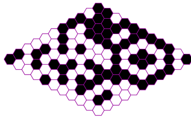
Fig. 5.3. A completed game.
