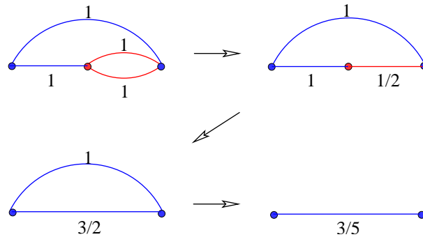
Fig. 3.6. A game on the network in the upper left corner, with resistances all equaling to 1, has the value 3/5
