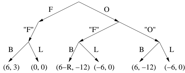
Fig. 4.16. The Kuhn tree for the fish-selling game.
