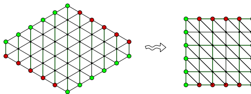
Fig. 2.18. Under T an equilateral triangular lattice is transformed to an equivalent lattice.
