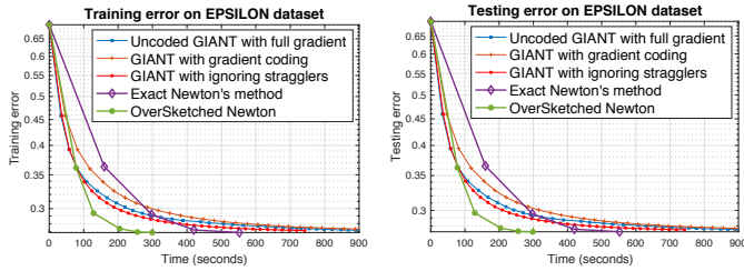
(a) Training error for logistic regression on EPSILON dataset (b) Testing error for logistic regression on EPSILON dataset
