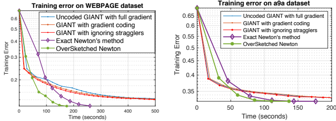
(a) Logistic regression on WEBPAGE dataset (b) Logistic regression on a9a dataset
