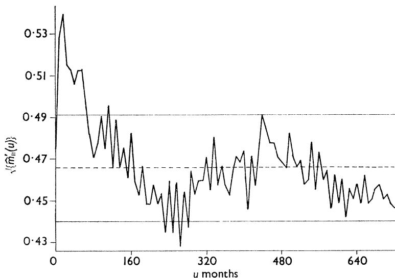
FIG. 2. Square root of the autointensity histogram of a sequence of times of major earthquakes.
