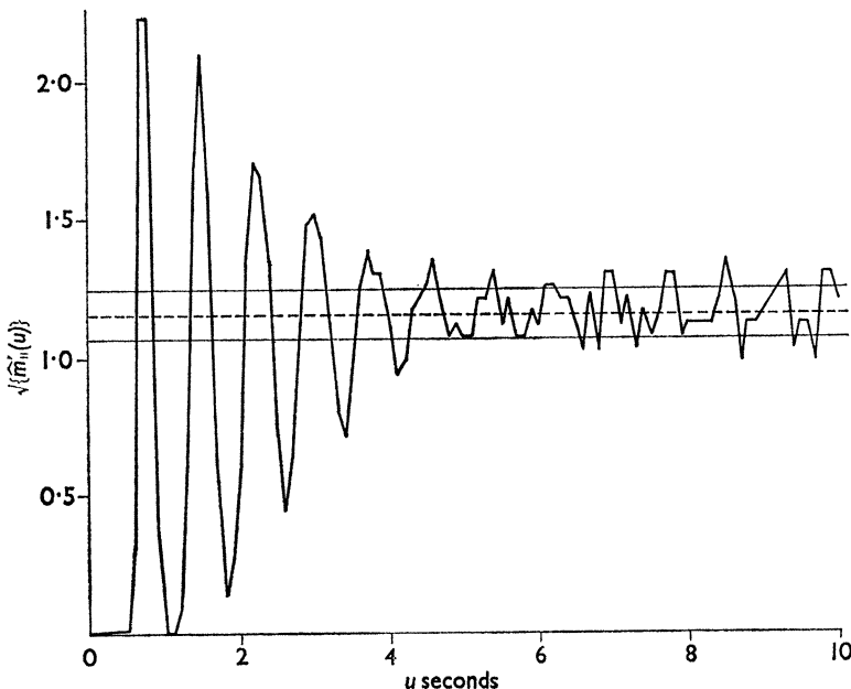
FIG. 1. Square root of the autointensity histogram of a sequence of times of heartbeats.
