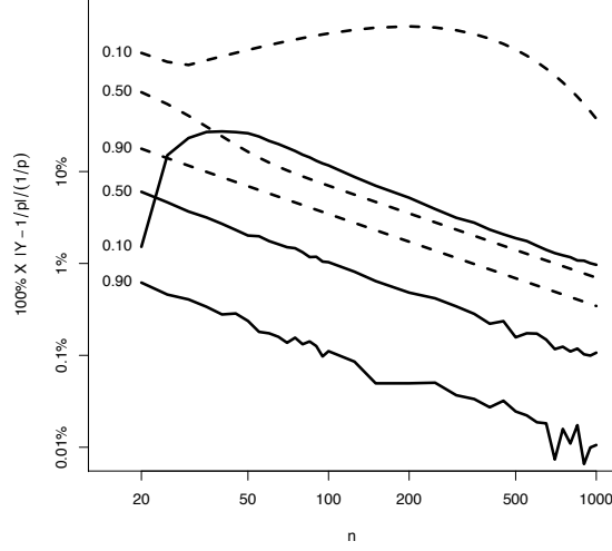
Figure 2: log-log plot comparing actual percent difference 100\% \times (\mathbb{E}[Y] - 1/p)/(1/p) , Y as defined in Lemma 10.2 to the given bound. Three probabilities of assignment shown: p = 0.1, 0.5 , and 0.9 . Actual differences computed with Monte Carlo. Y generated with Bernoulli distribution.
