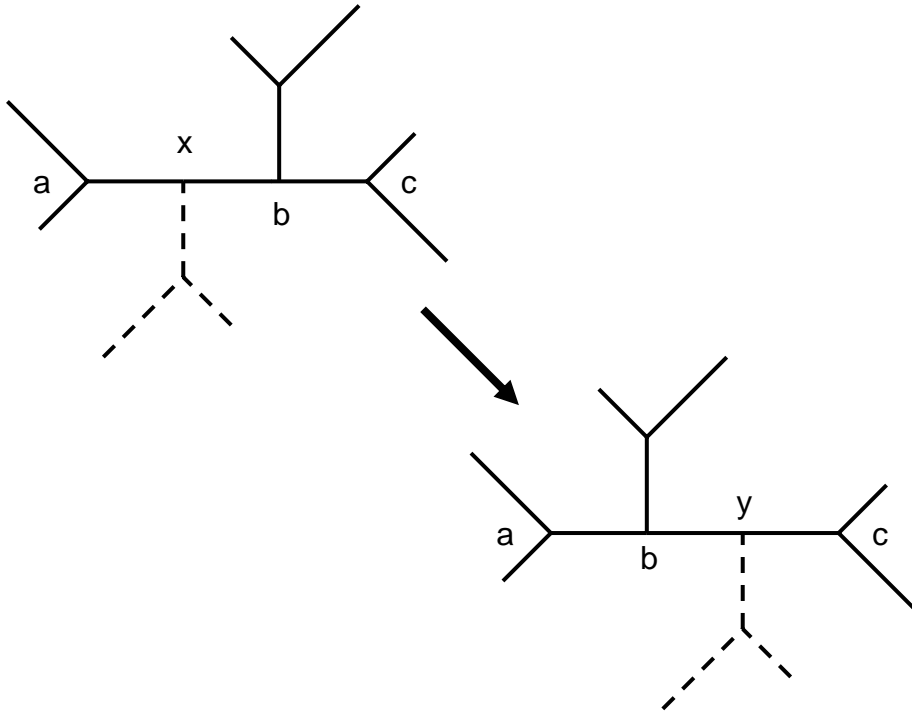
FIGURE 1. An SPR move. The dashed subtree tree attached to vertex x in the top tree is re-attached at a new vertex y that is inserted into the edge (b, c) in the bottom tree to make two edges (b, y) and (y, c) . The two edges (a, x) and (b, x) in the top tree are merged into a single edge (a, b) in the bottom tree.
