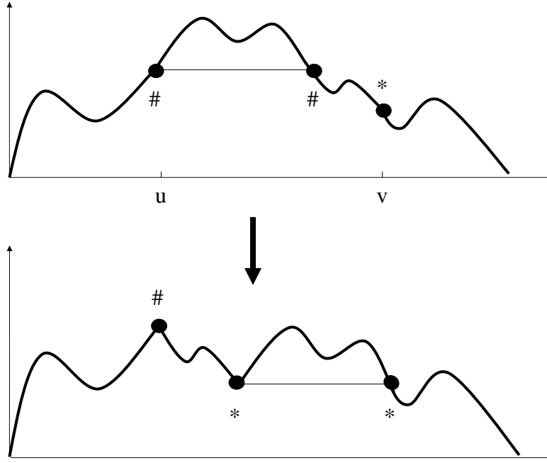
FIGURE 2. A subtree prune and re-graft operation on an excursion path: the excursion starting at time u in the top picture is excised and inserted at time v , and the resulting gap between the two points marked \# is closed up. The two points marked \# (resp. * ) in the top (resp. bottom) picture correspond to a single point in the associated \mathbb{R} -tree.
