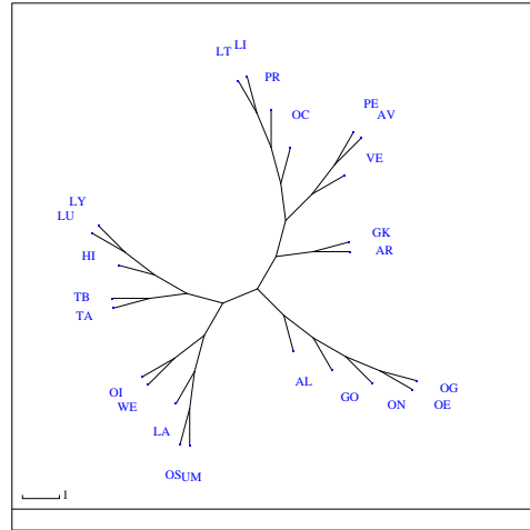
(b) T_{WMC}
