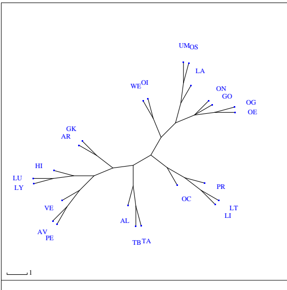
(a) LT_{MP}
