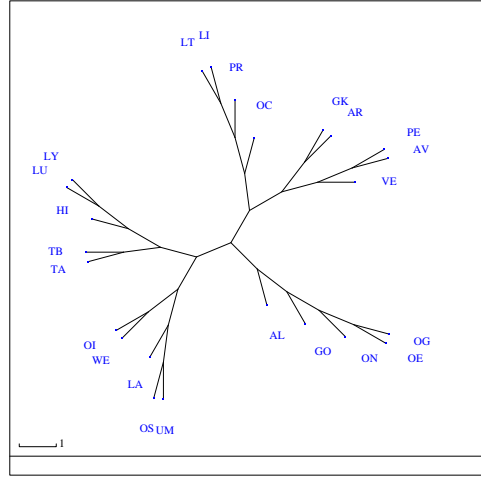
(b) T_{WMC}
