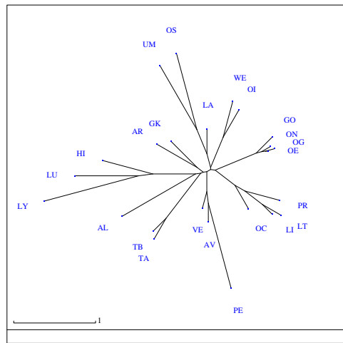
(e) T_{NJ}
