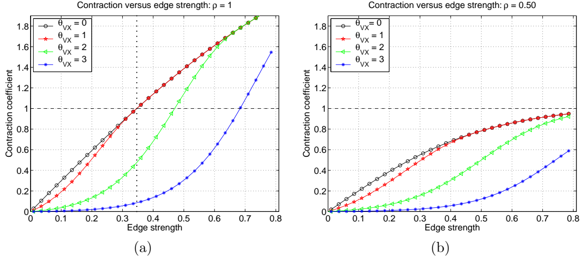
Figure 2. Plots of the contraction coefficient R_4(\theta_{vx}, \theta_{ed}; \rho) versus the edge strength \theta_{ed} . Each curve corresponds to a different choice of the observation potential \theta_{vx} . (a) For \rho = 1 , the updates reduces to the standard sum-product algorithm; note that the transition from convergence to non-convergence occurs at \theta_{ed}^* \approx 0.3466 in the case of no observations ( \theta_{vx} = 0 ). (b) Corresponding plots for reweighted sum-product with \rho = 0.50 . Since \rho d = (0.50)4 = 2 , the contraction coefficient is always less than one in this case, as predicted by Proposition 1.
