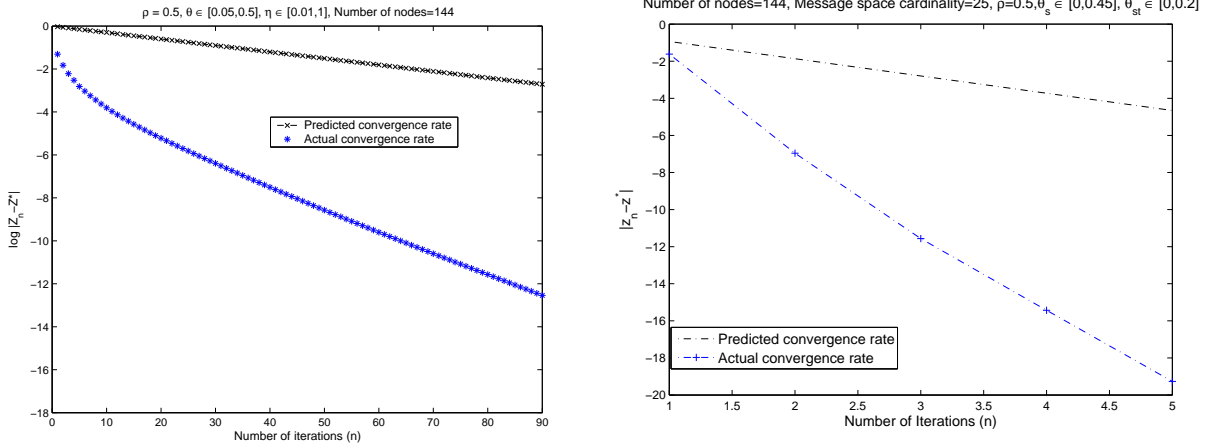
Figure 4. Convergence rates of the reweighted sum-product algorithm as compared to the rate predicted by reweighted norm condition 19. (a) Binary state spaces ( m = 2 ). (b) Higher-order spaces ( m = 25 ).
