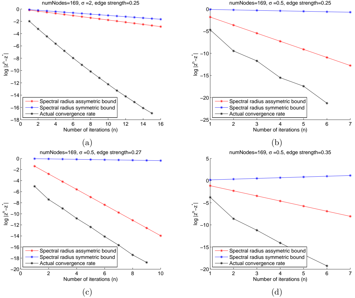
Figure 5. Empirical rates of convergence of the reweighted sum-product algorithm as compared to the rate predicted by the symmetric and asymmetric bounds from Theorem 2.
