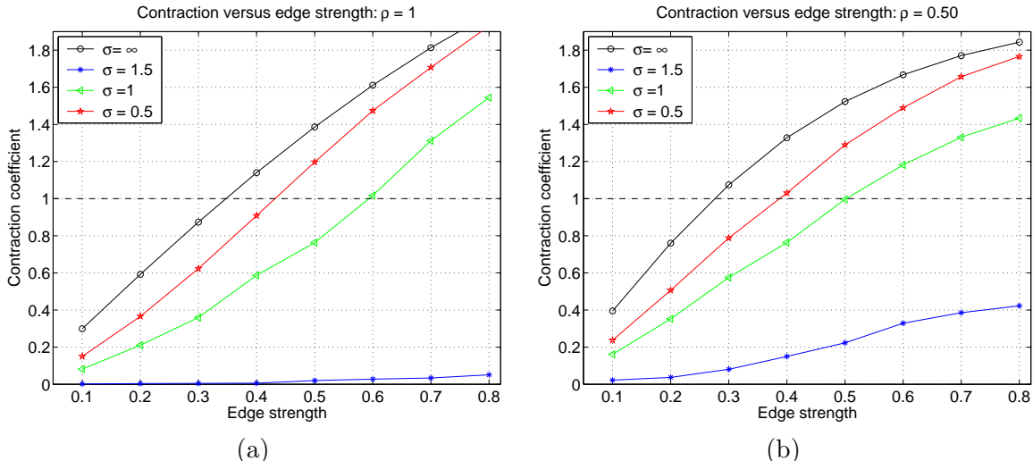
Figure 3. Illustration of the benefits of observations. Plots of the contraction coefficient versus the edge strength. Each curve corresponds to a different setting of the noise variance \sigma^2 as indicated. (a) Ordinary sum-product algorithm \rho = 1 . Upper-most curve labeled \sigma^2 = +\infty corresponds to the best bounds from previous work [14, 15]. (b) Reweighted sum-product algorithm \rho = 0.50 .
