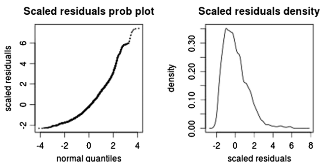
Figure 7. The left-hand plot here provides a normal quantile plot, and the right hand, a density estimate of the scaled residuals
