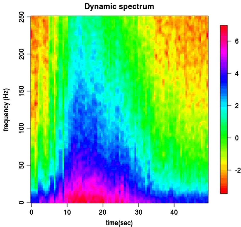
Figure 17. Spectrogram of the time series of Figure 3
